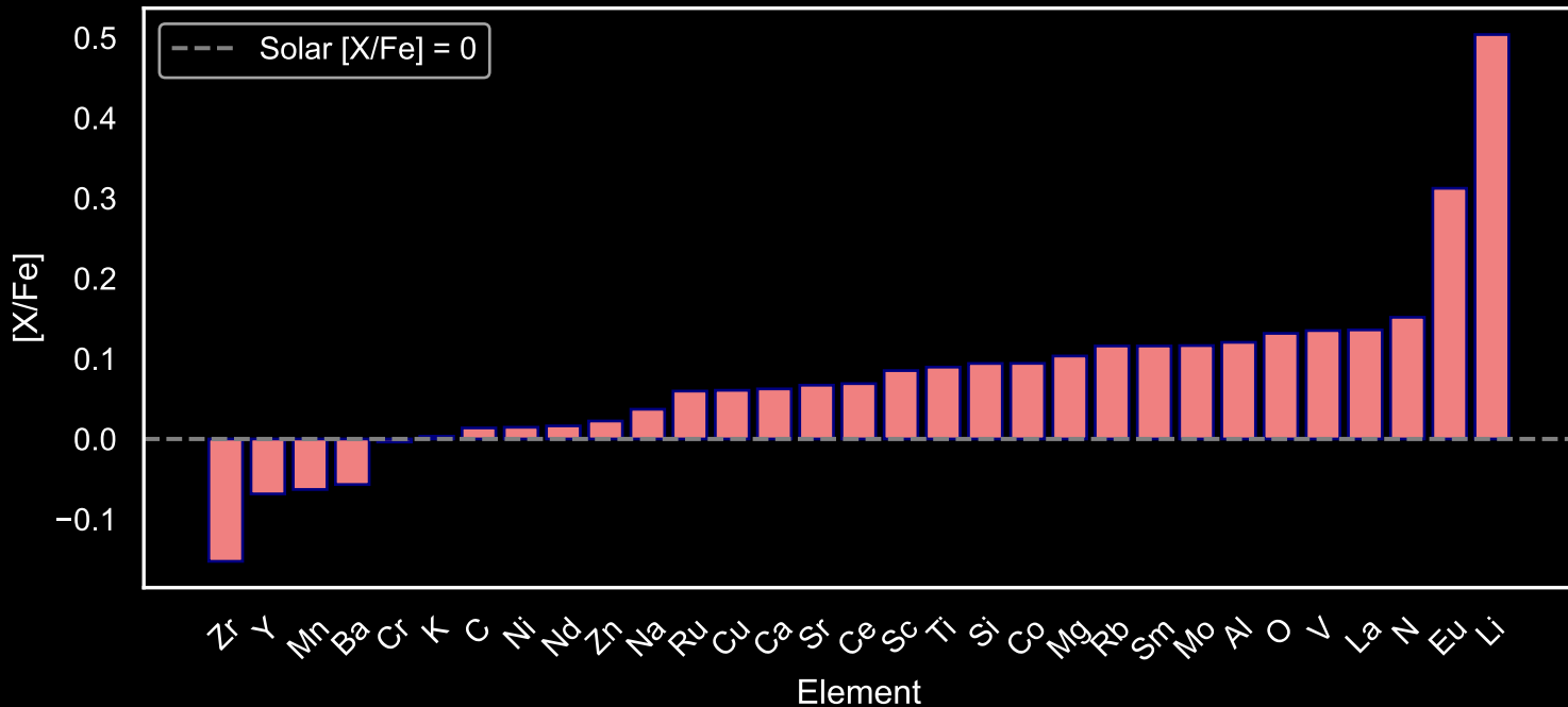
Abundance Pattern for GALAH Star Field [116] (N=284)
