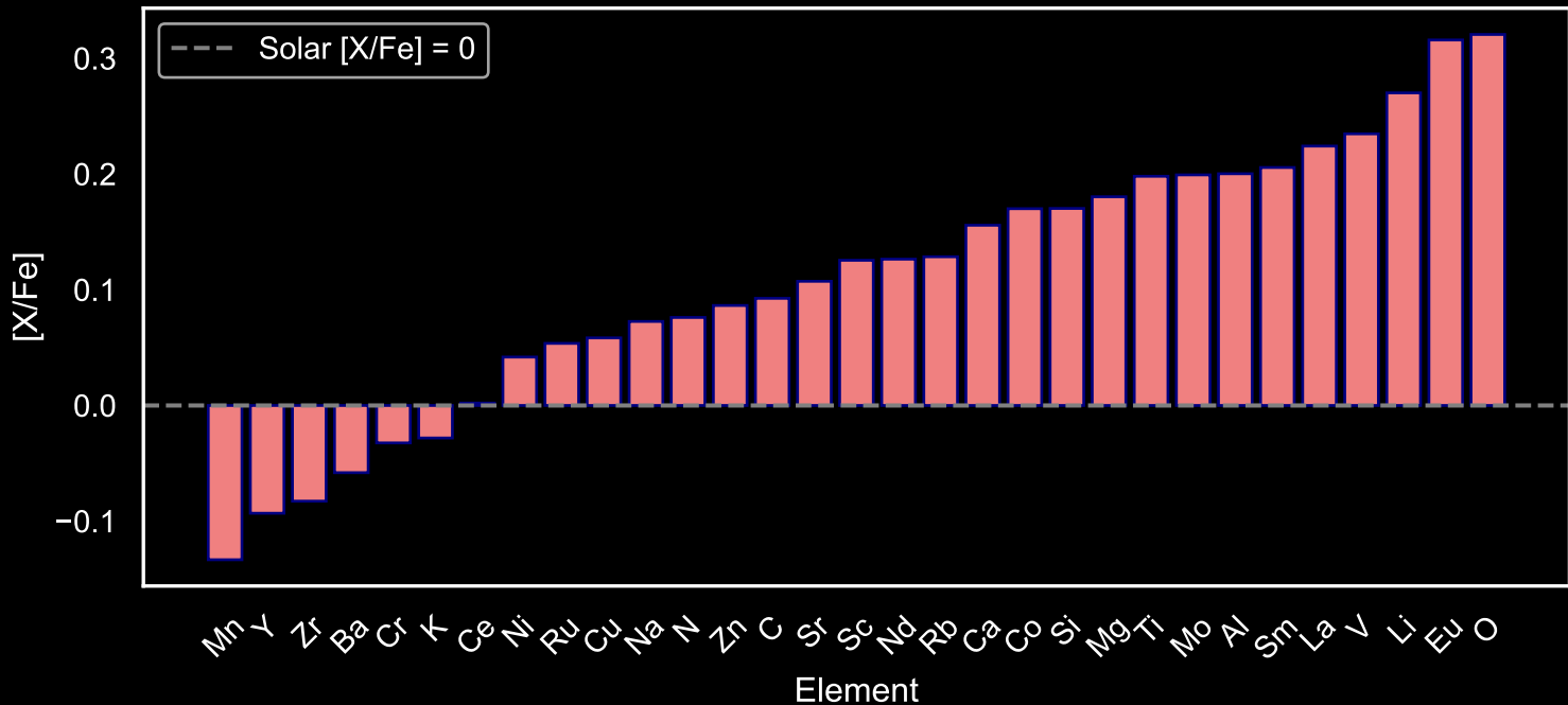
Abundance Pattern for GALAH Red Giants: Star Field [116] (N=65)
