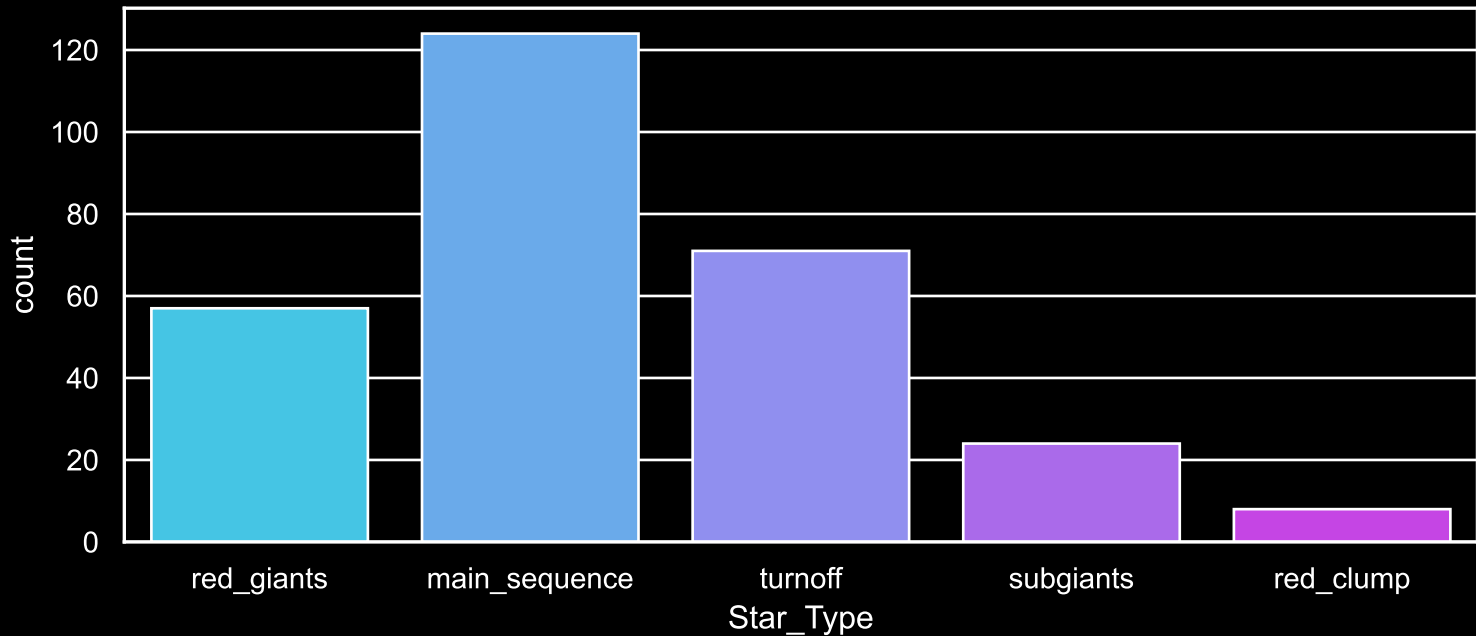
Field [116] Count plot of Star Type
