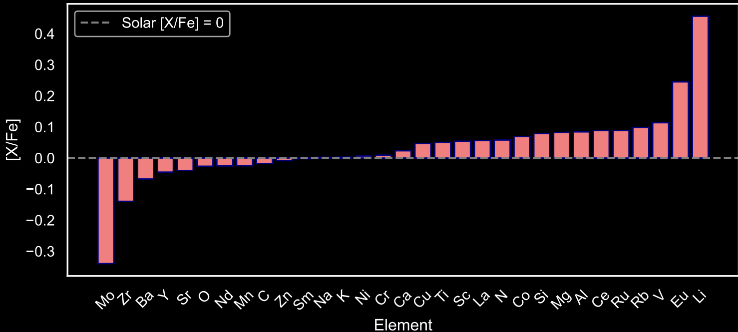
Abundance Pattern for GALAH Main Sequence Stars: Star Field [116] (N=124)
